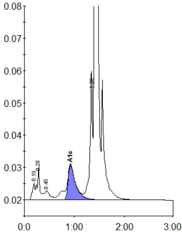
Peak table - ID: 10484549
